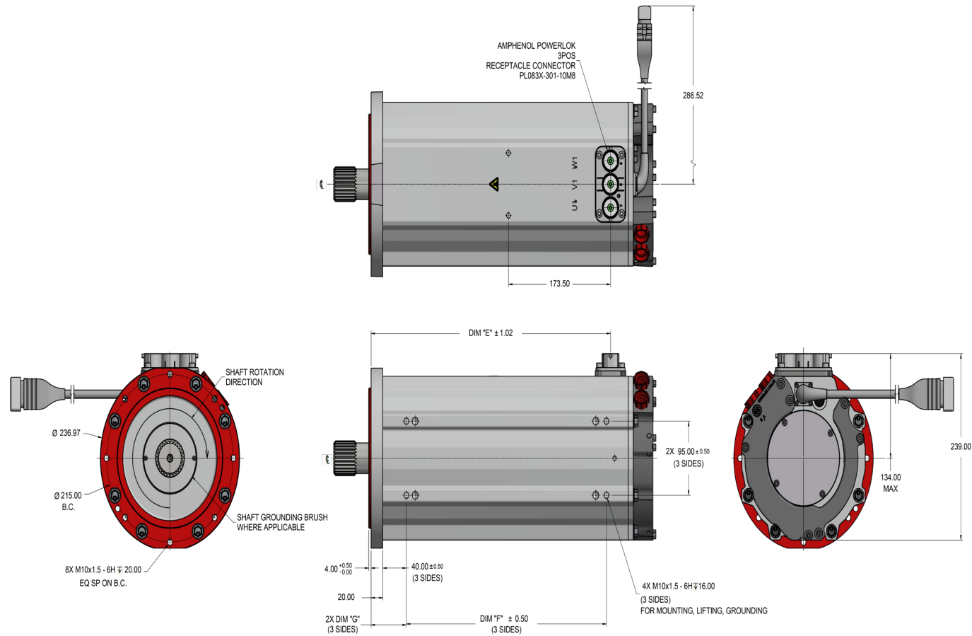
Power connector option 3 - 1 x HV PowerLok™ 300A
